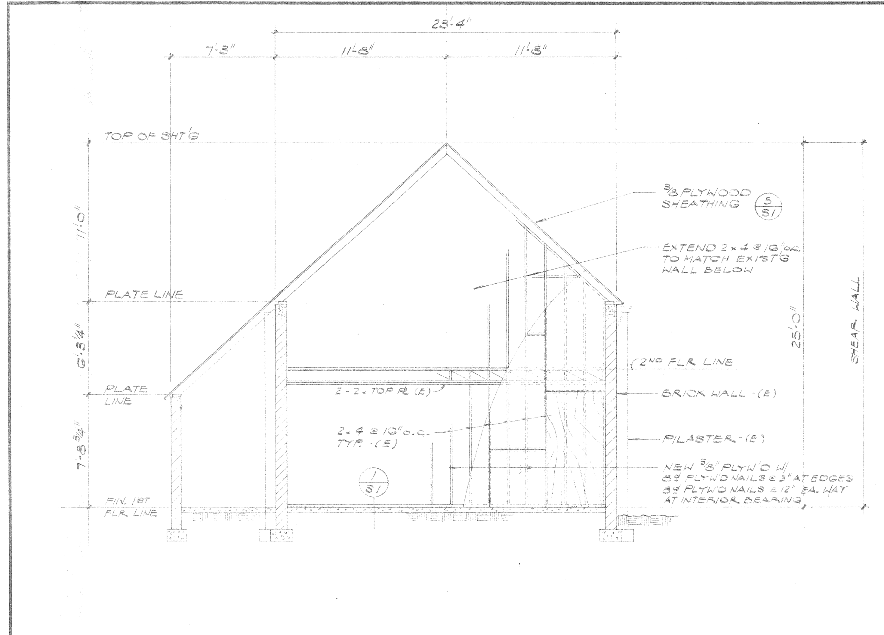
SHEAR WALL ELEVATION
