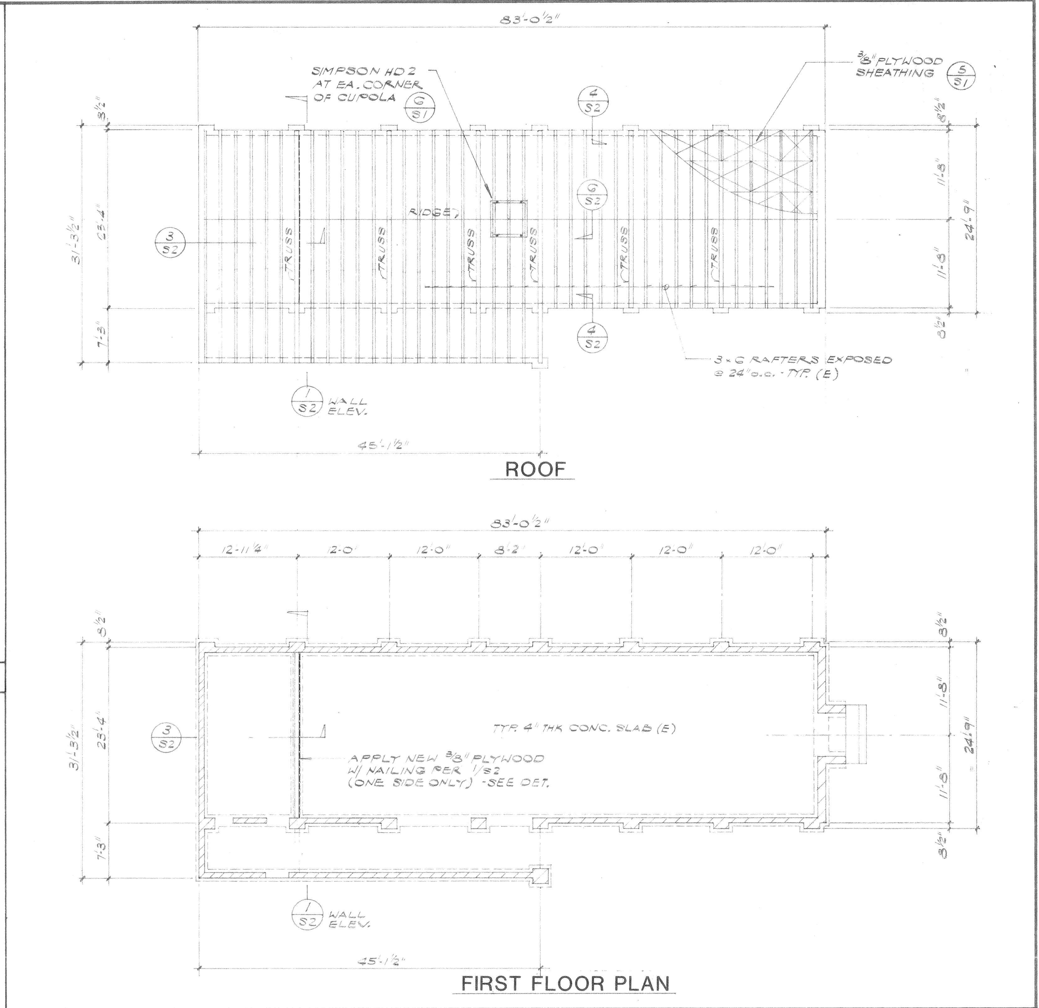
PLAN OF ROOF & FIRST FLOOR
